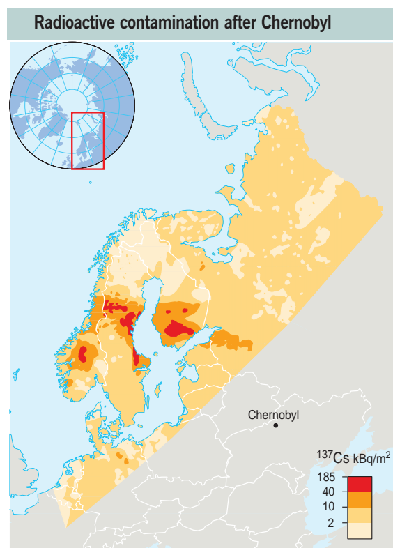
Levels of caesium 137 (1 000 becquerels/m 2 ) in Scandinavia, Finland and the Leningrad region of Russia following the Chernobyl explosion in 1986
