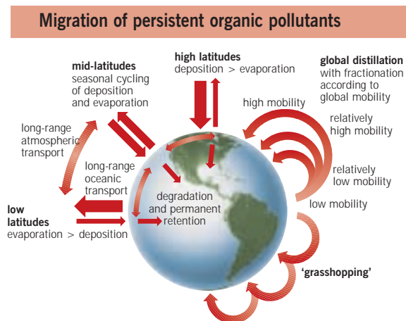
Persistent organic pollutants spread via a variety of mechanisms at different latitudes
