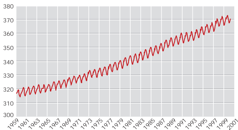
Carbon dioxide concentrations at Mauna Loa, Hawaii (parts per million by volume)
